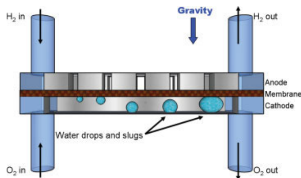
Figure 6. Schematic of the horizontal fuel cell with the cathode facing down (H-i).
